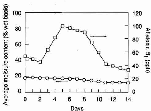
Figure 11. Changes in average moisture content and aflatoxin B 1 concentration at 30 cm depth in bulk maize versus drying time (initial moisture content = 18.7% wet basis).
