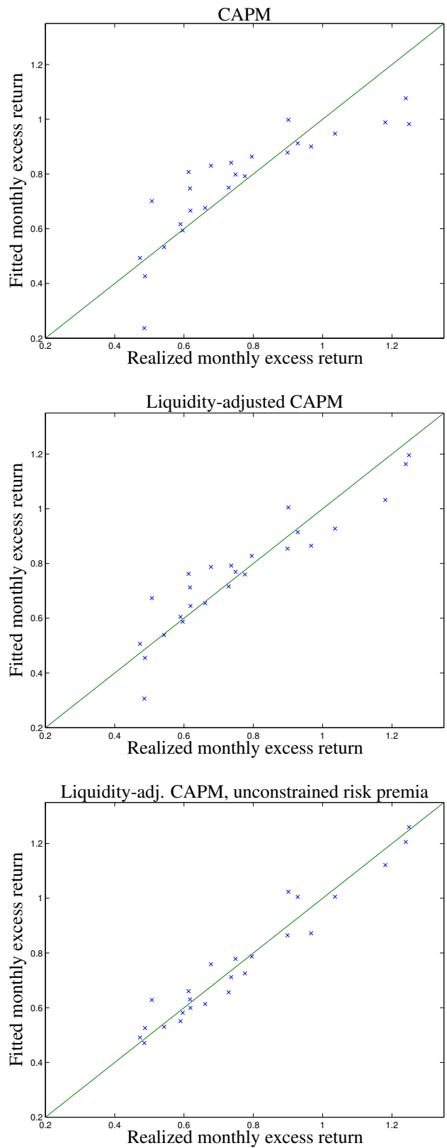
Figure 3: \sigma (illiquidity) portfolios: The top panel shows the fitted CAPM returns vs. realized returns using monthly data 1964–1999 for value-weighted \sigma (illiquidity) portfolios. The middle panel shows the same for the liquidity-adjusted CAPM, and the lower panel shows the relation for the liquidity adjusted CAPM with unconstrained risk premia.
