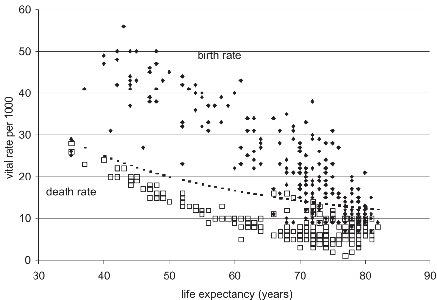
Figure 1: Crude birth rate (filled diamonds) and crude death rate (open squares) (annual, per 1000) as a function of life expectancy (years) for both sexes combined in 222 countries or territories
