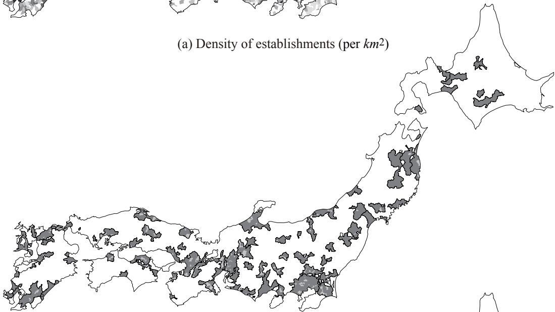
(b) Clusters
