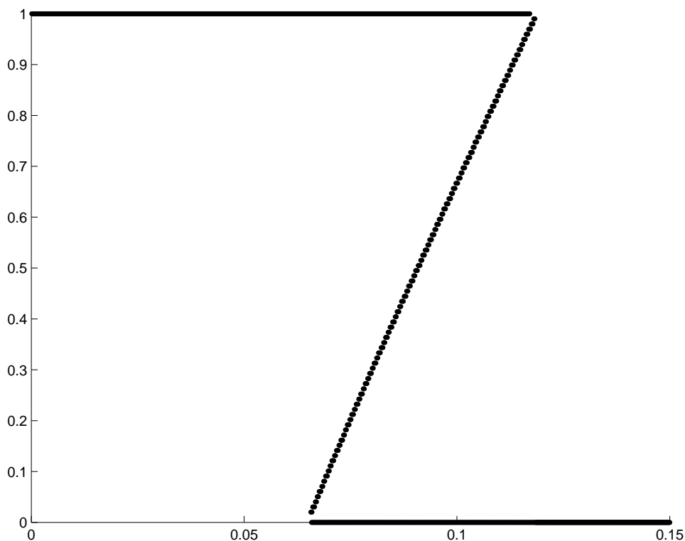
Figure 2: Bifurcation Diagram.
