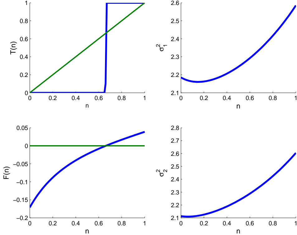
Figure 1: Multiple Misspecification Equilibria.
