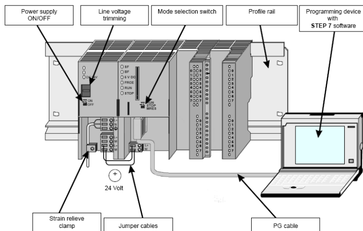
Figure 1. Structure of automation system Siemens S7-300
