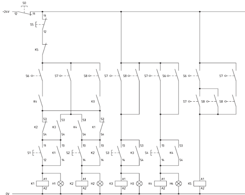
Figure 5. Current flow for functional description b
