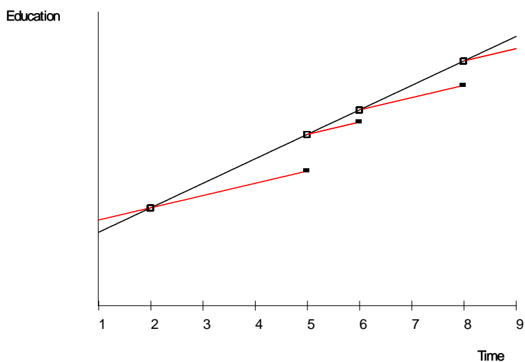
Figure 1: Plot of education with census and non-census data
