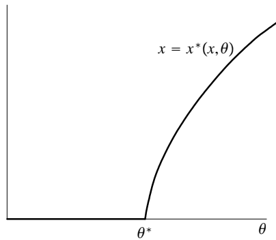
Fig. 8: NEC, \partial x^*(0, \theta^*)/\partial k \leq 1 , concave RCs
