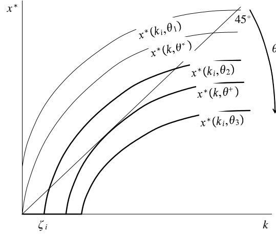
Figure 3: NE at fixed values of \theta , \frac{\partial x^*}{\partial k_i}(0, \theta^*) > 1
