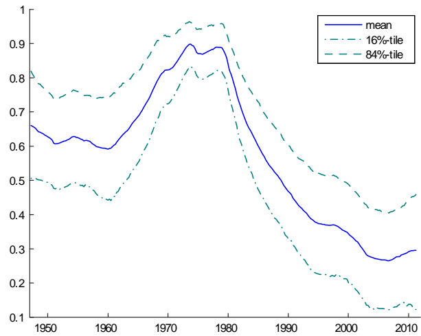
Figure 7: Posterior mean and quantiles of \rho_t under the AR-trend-bound model.
