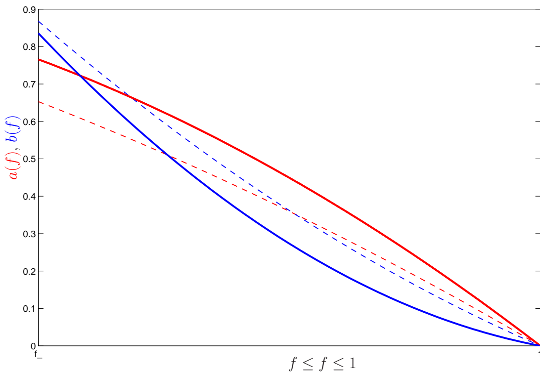
Figure 1: Equilibrium Reelection Probabilities for \mu = 50 (solid lines) and \mu = 25 (dashed lines). Other parameter values: M = 100 , \rho = 0.8 , q = 0.56 .
