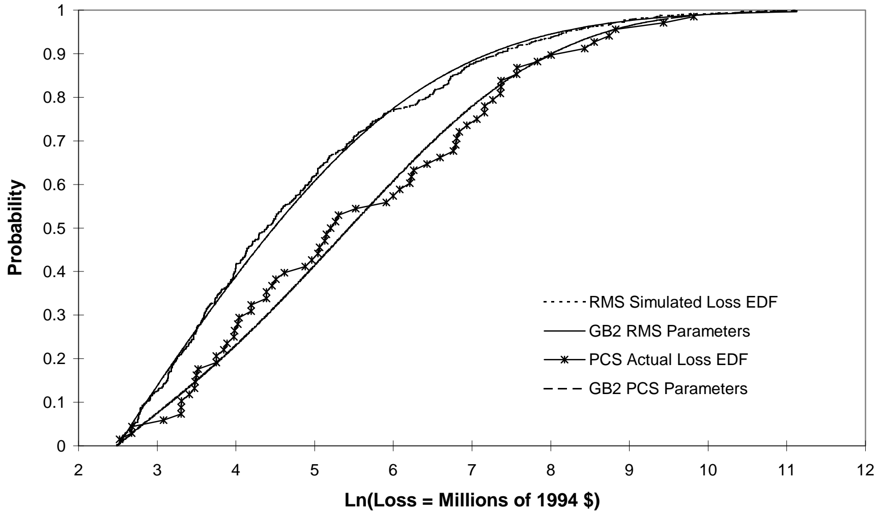
Figure 6: Fitting Severity Loss Distribution Functions: GB2 Hurricane and Earthquakes PCS Reported Actual Losses Vs. RMS Simulated Losses
