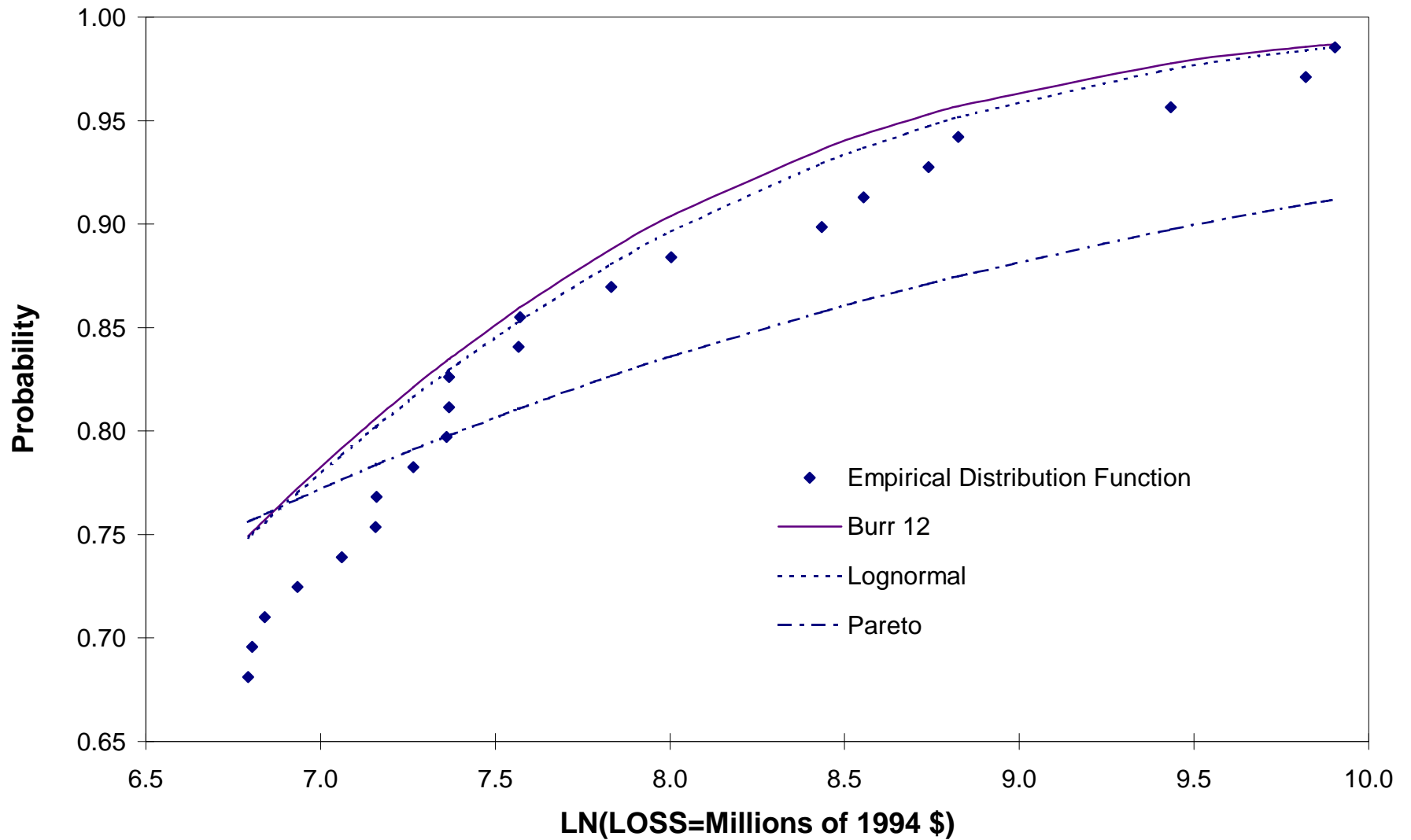
Figure 4: Severity of Loss Distribution Function Tails: Earthquakes and Hurricanes
