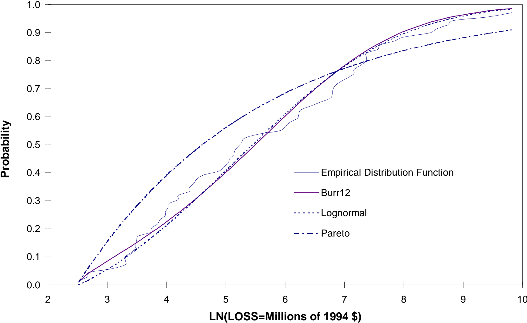
Figure 3: Severity of Loss Distribution Functions: Earthquakes and Hurricanes
