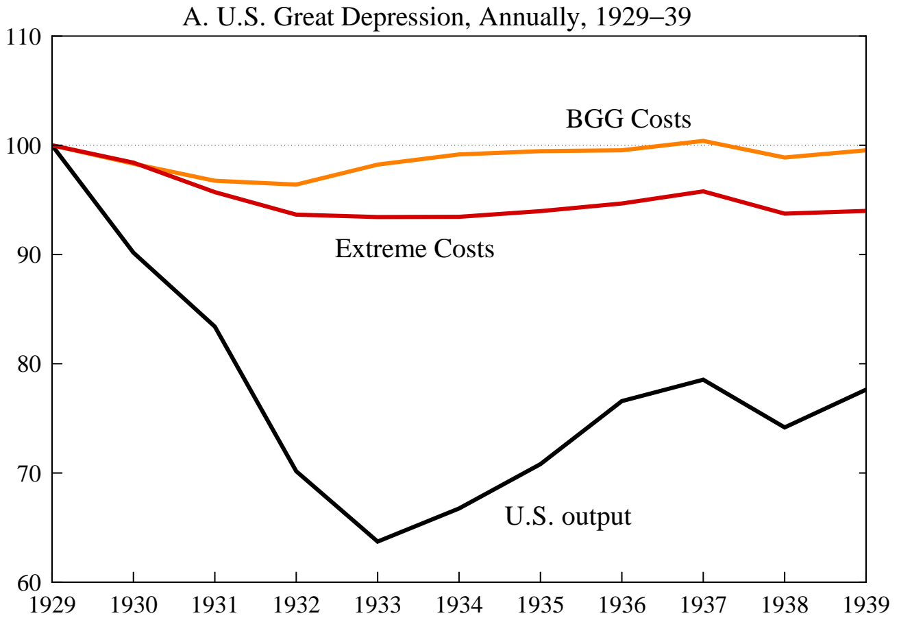
Figure 14. U.S. Output and Predictions of Model With Alternative Adjustment Costs and Just the Investment Wedge (Normalized to Equal 100 in 1929 or 1979:1)
