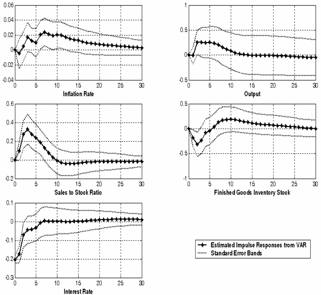
Figure 1: Estimated Impulse Responses from a VAR Model
