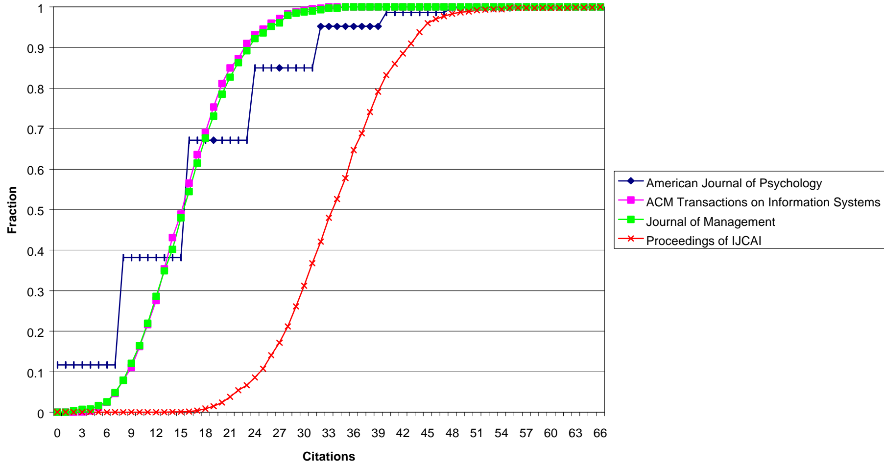
Figure 3: Classifying outliers
