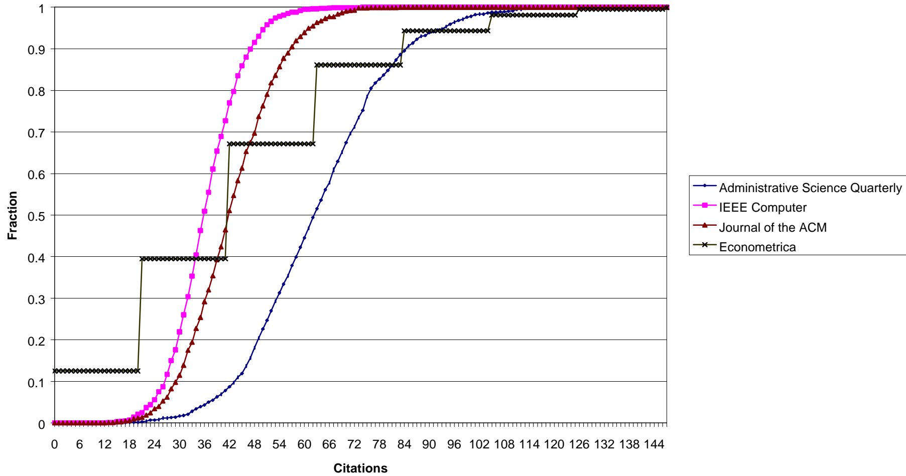
Figure 2: Detecting outliers
