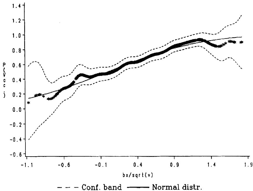
Figure 1. P(Vac.) from Probit and non-parametric regression
