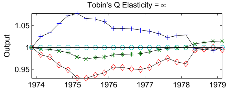
Figure A2: Raw Data ('all wedges') and Various Counterfactual Simulations
