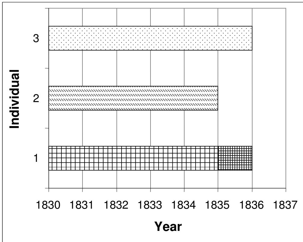
Figure 2: Genuine and Synthetic Longitudinal Measurements
