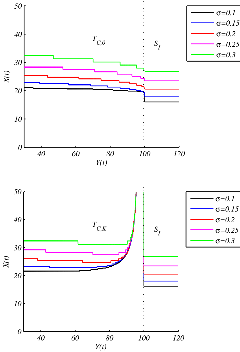
Figure 3: The comparative statics with respect to the volatility \sigma . The upper and lower panels illustrate the cases with only a proportional cost and both fixed and proportional costs, respectively. The parameter values other than \sigma are set at the base case (21).
