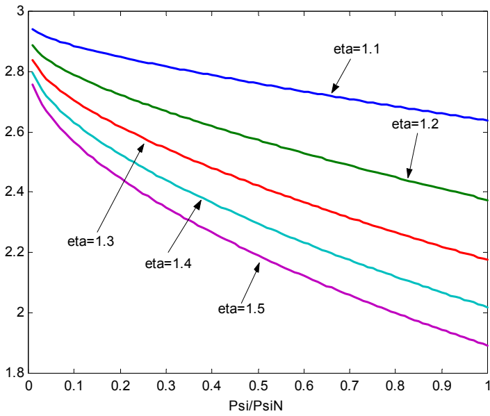
Figure 3: \rho(\psi/\psi_N|\eta)
