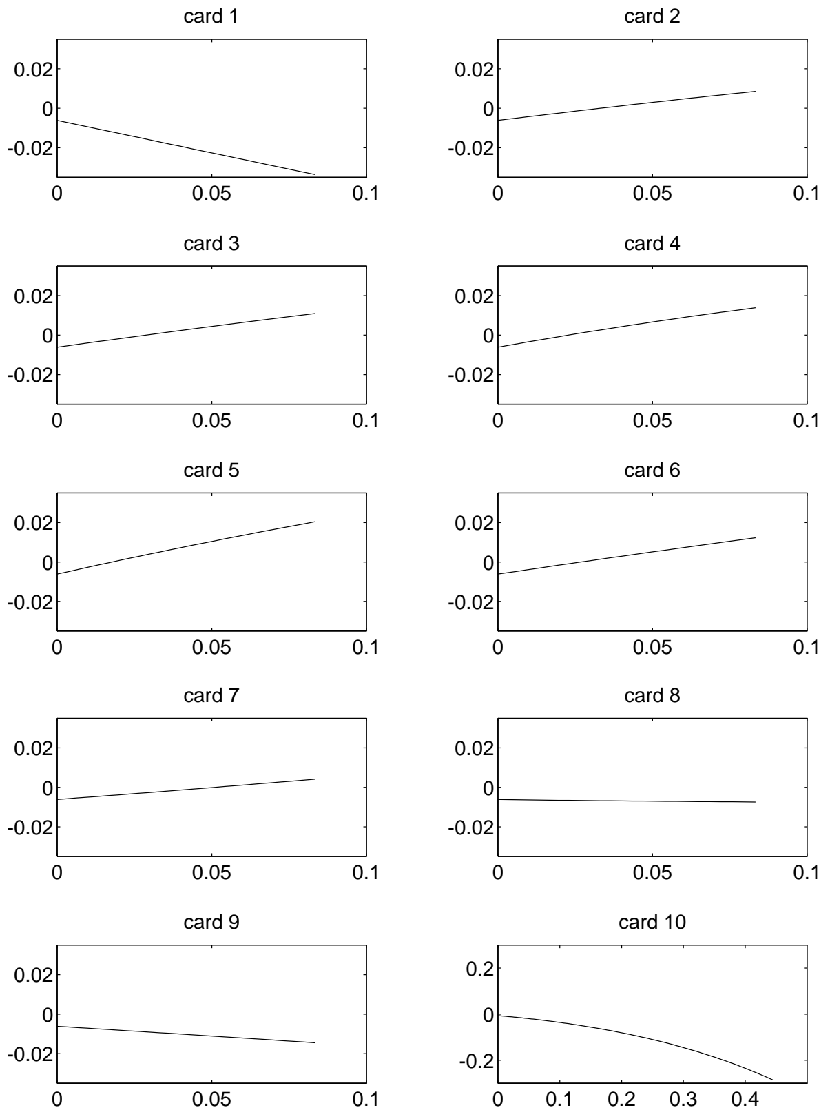
Figure 20. E(G_1(c)) for card fractions F_j(t) w.r.t S_{bas} using BJ1ISTR1.
