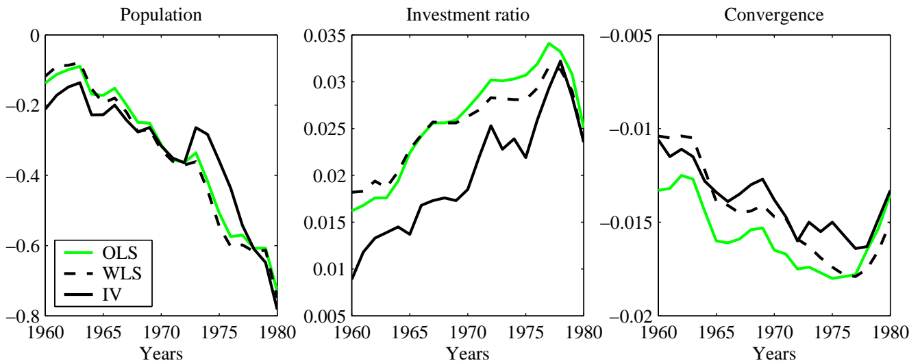
Figure 4: Rolling regressions
