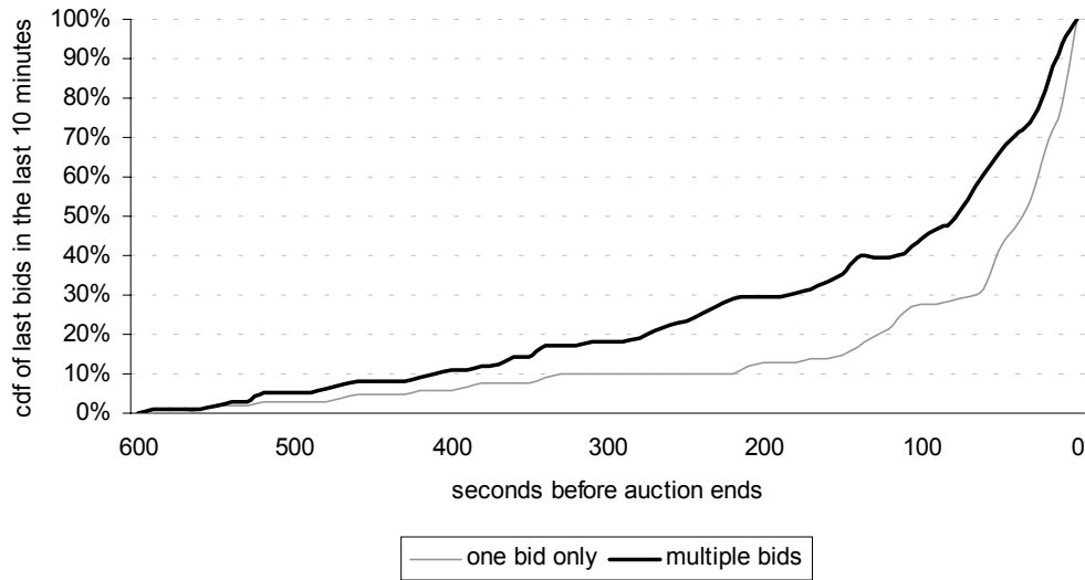
Figure 4. Cumulative distribution functions of last bids within the last ten minutes for bidders with one bid and for bidders with multiple bids
