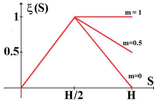
Figure 3: Asymmetric peaked function for some values of m .
