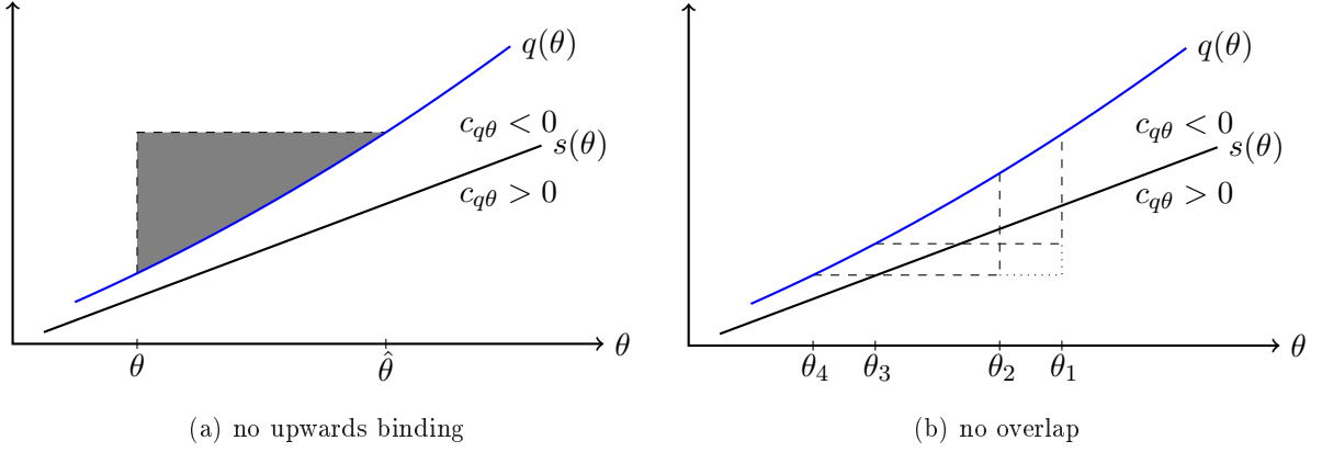
Figure 4: non-binding constraints
