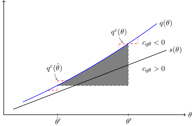
Figure 6: feasible changes
