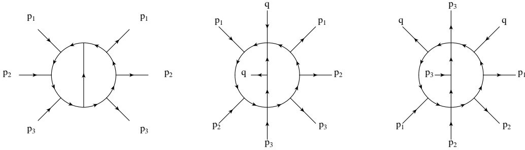
Figure 1: The planar and two non-planar auxiliary diagrams. All nine possible dot-products involving the loop momenta and the external particle momenta are mapped onto the nine propagators.
