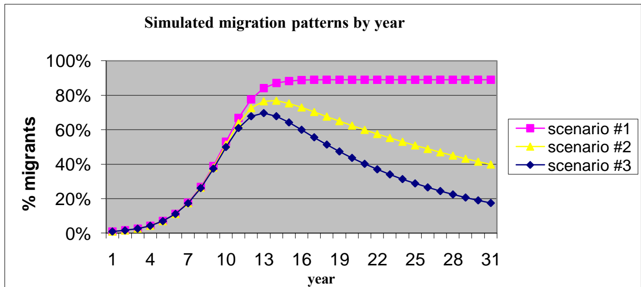
Figure 4: Simulated migration
