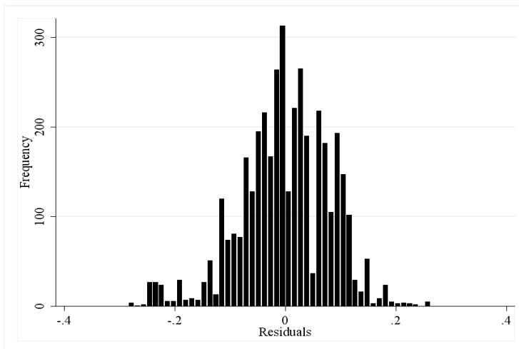
Figure 4: Simulated migration
