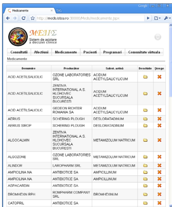
Fig. 3. Medicine management
