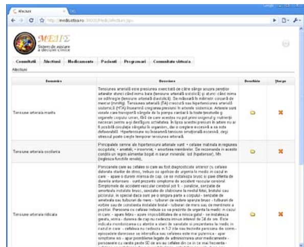
Fig. 4. Treatment management
