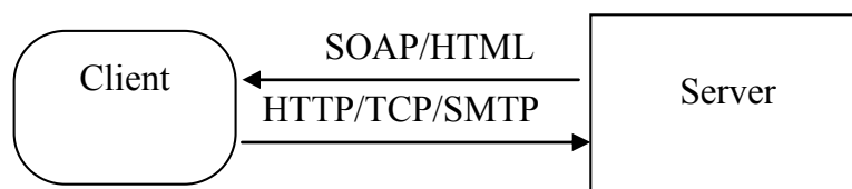
Fig.1. Web Services
