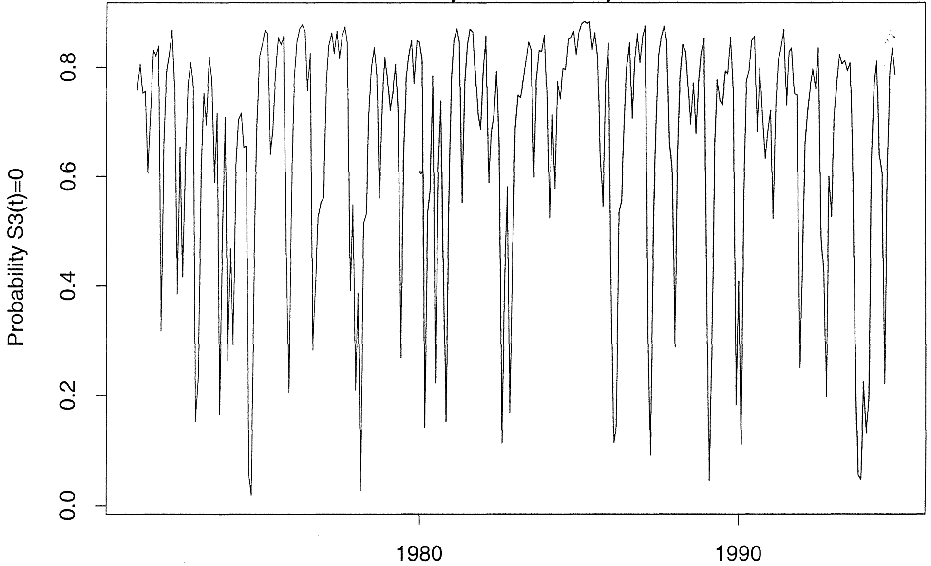
Probability of Low Volatility State
