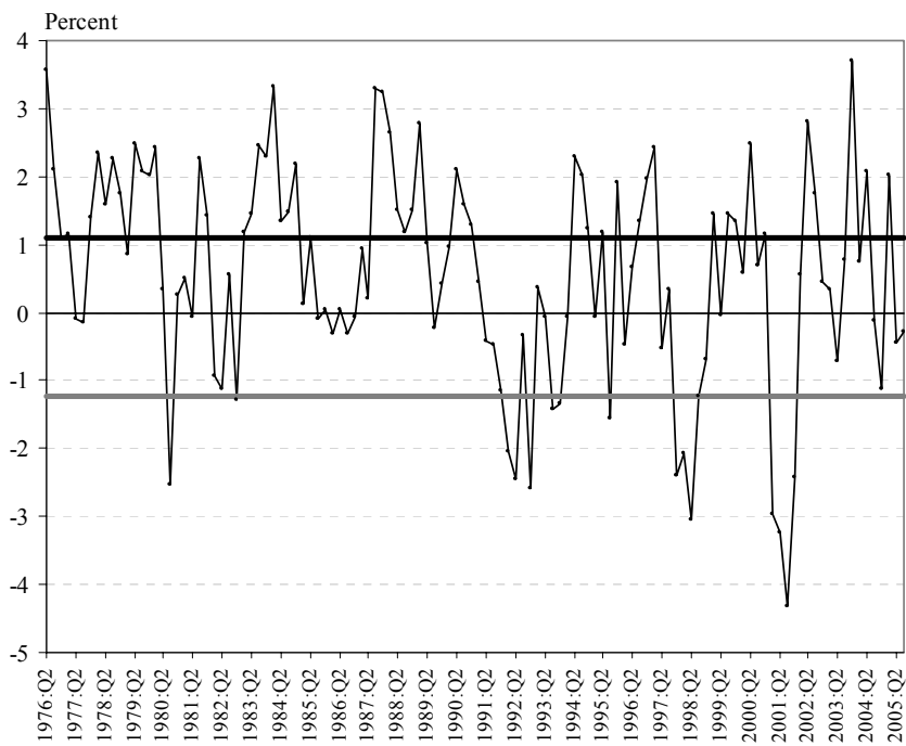
Figure 1 Growth of IIP: Japan, No Structural Break Thick black line is expansion growth rate; thick gray line is recession growth rate.
