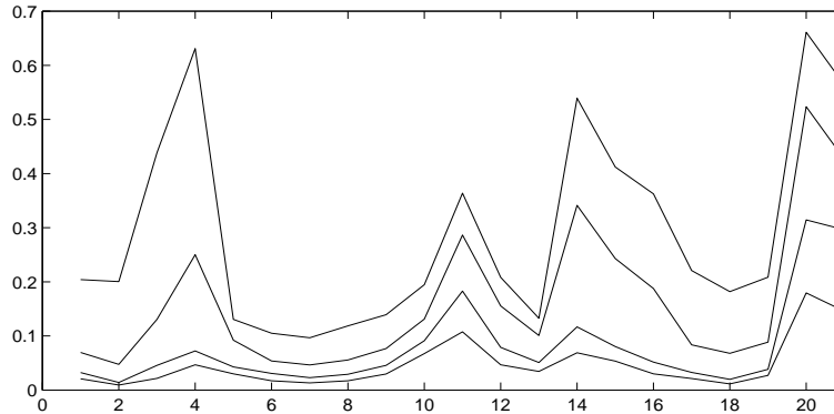
Figure 3.2 Variance-ratio of idiosyncratic component to the variable
