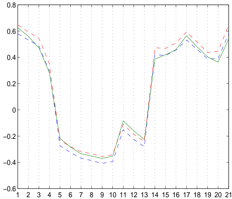
Figure 5.1 Estimated a_{i1,0} , solid line, and confidence bands, dashed line. Whole period.
