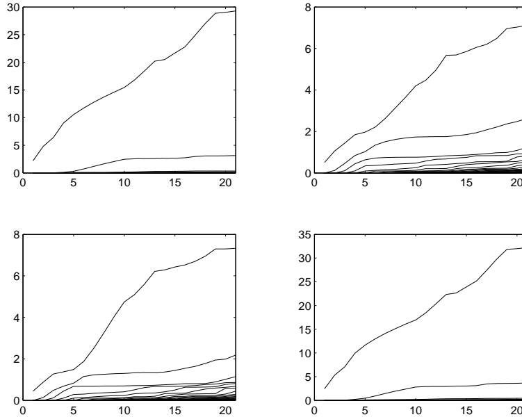
The graphs in the first row, from the left, correspond to the frequencies 0, \pi/3 , in the second row to 2\pi/3, \pi .
