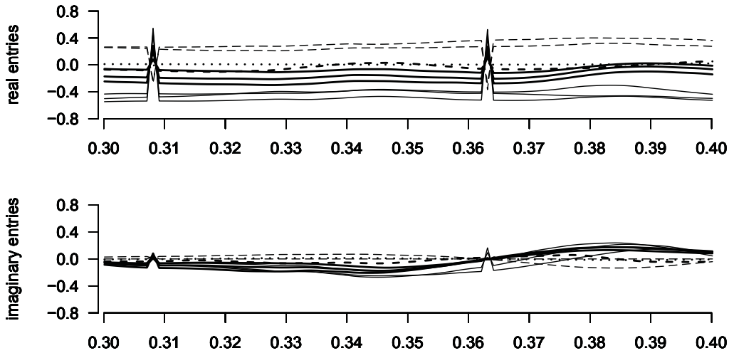
Figure 2: Real and imaginary parts of the entries of the 10–dimensional complex eigenvectors without rotation over a range of 100 Fourier frequencies for one patient, HR and pulse ( dashed ), arterial blood pressures ( solid ), pulmonary artery pressures ( bold solid ), CVP ( bold dashed ), TEMP ( dotted )
