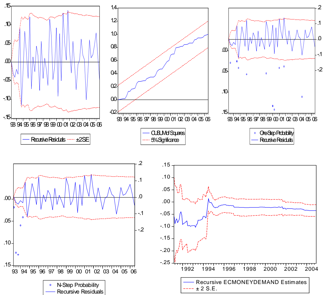
FIGURE 3: RESURSIVE ESTIMATES OF THE VEC MODEL UPON MONEY DEMAND
