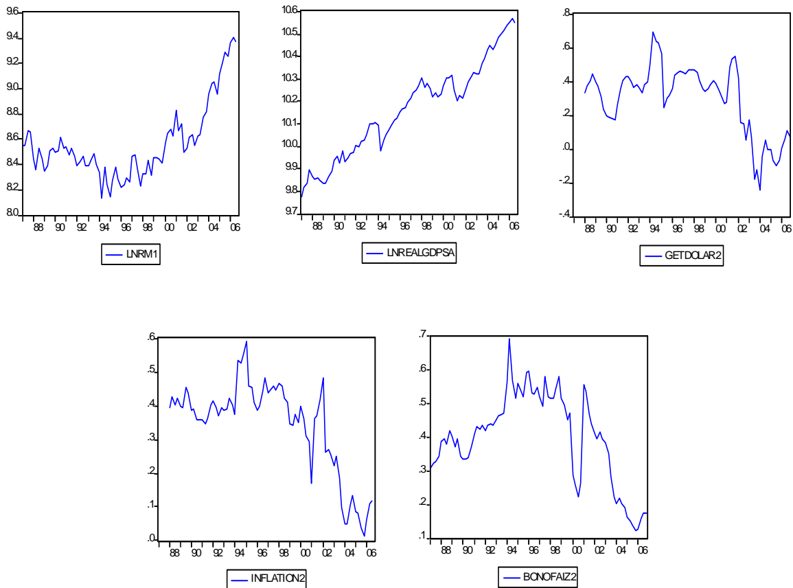
FIGURE 1: TIME SERIES USED IN THE PAPER
