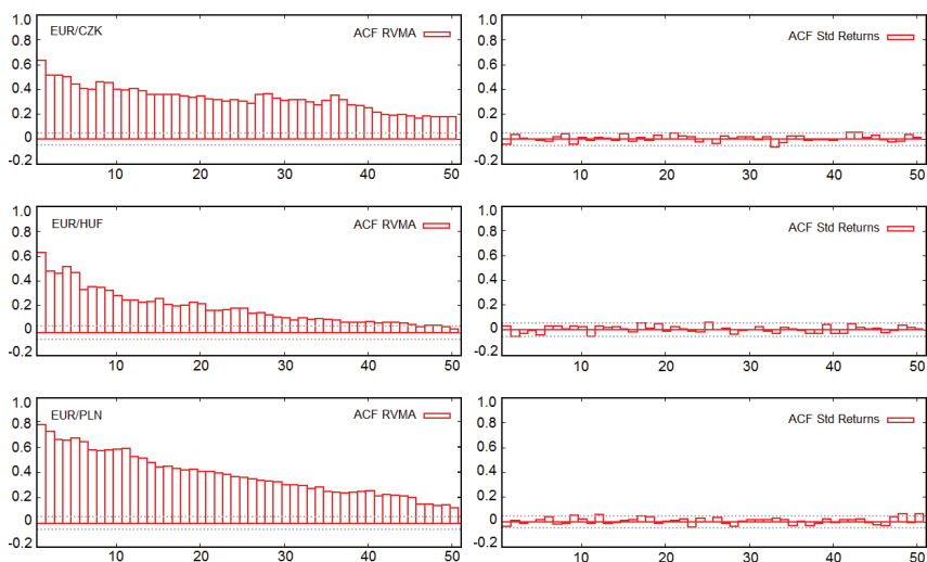
Figure 4 ACF Plots of Daily Realized Variance (RV), left, and of Daily Standardized Returns ( r/(RV)^{1/2} ), right for the case of EUR/CZK (first row), EUR/HUF (second row), and EUR/PLN exchange rate returns (third row)
