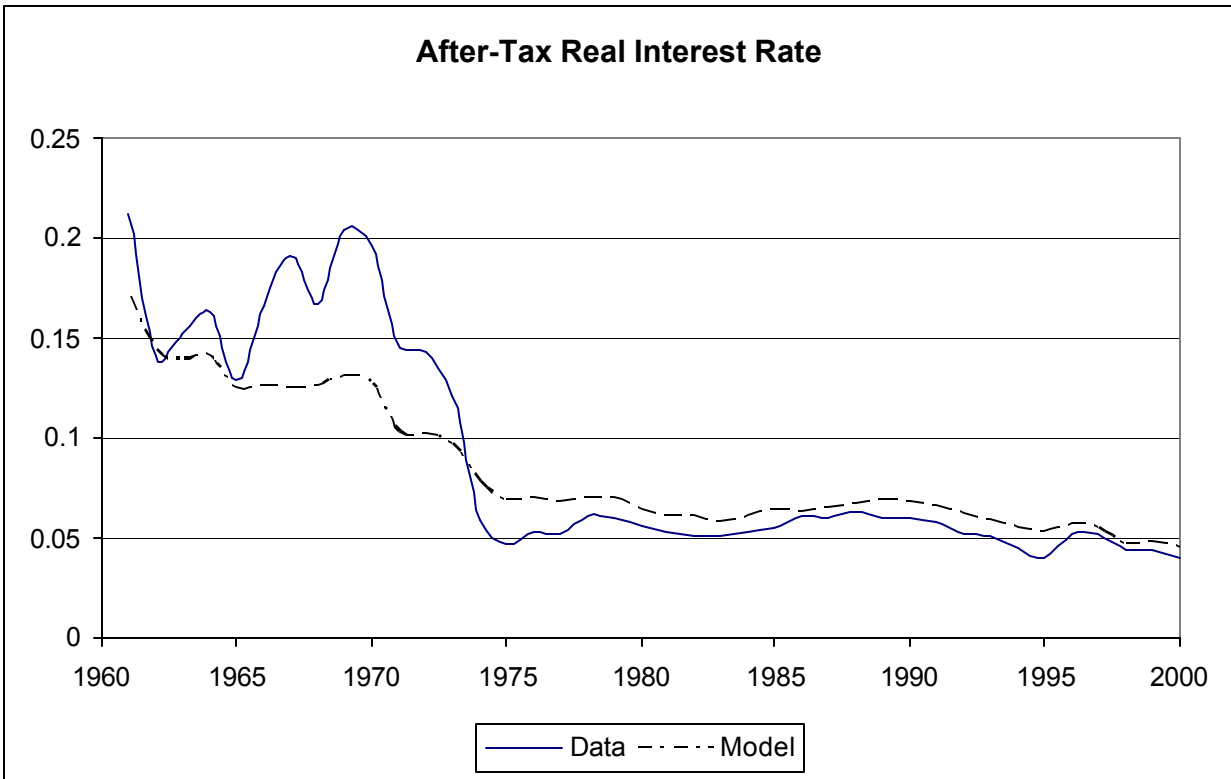
Figure 2: In-Sample Performance
