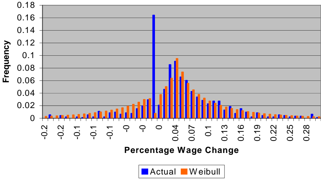
Figure A-3 2-Sided Weibull vs. Actual for US 97
