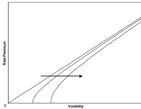
Figure 3: Mean-variance frontiers with and without background risks.
