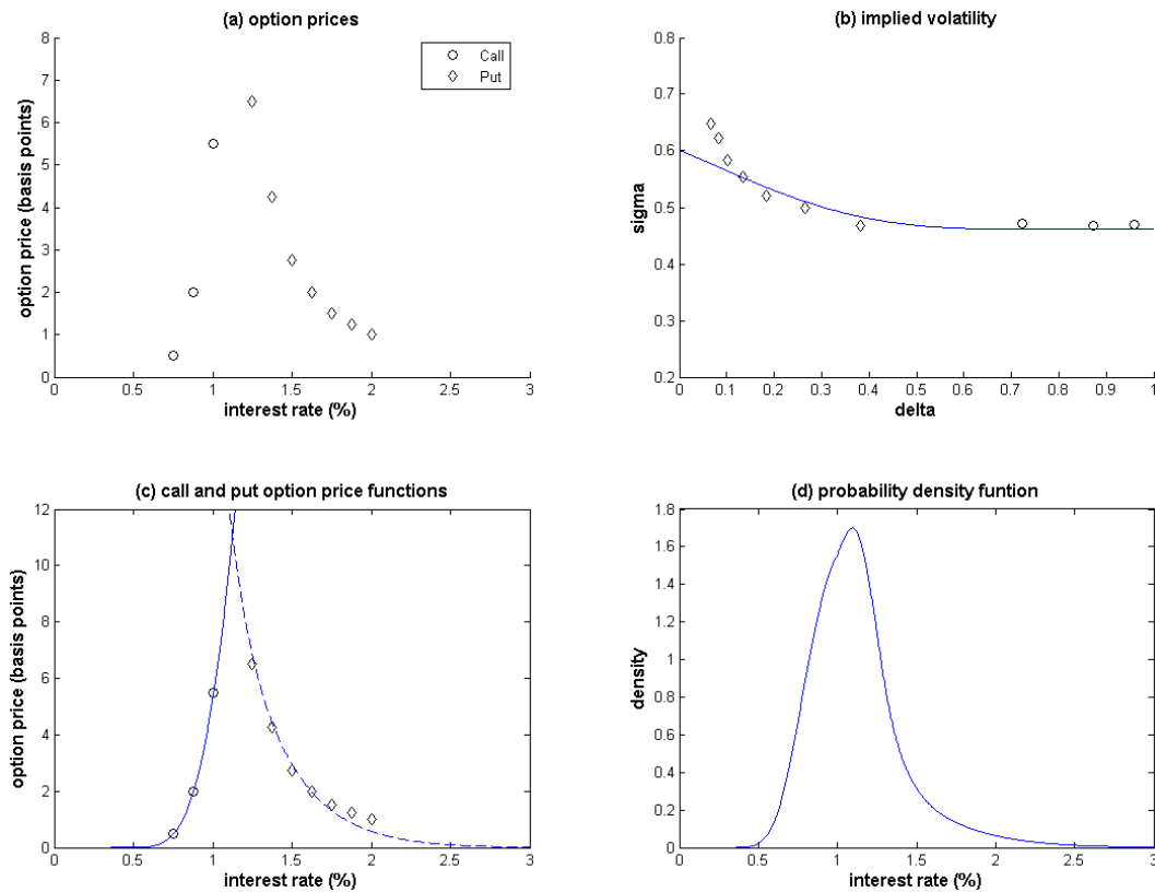
Figure 1: Estimation steps
