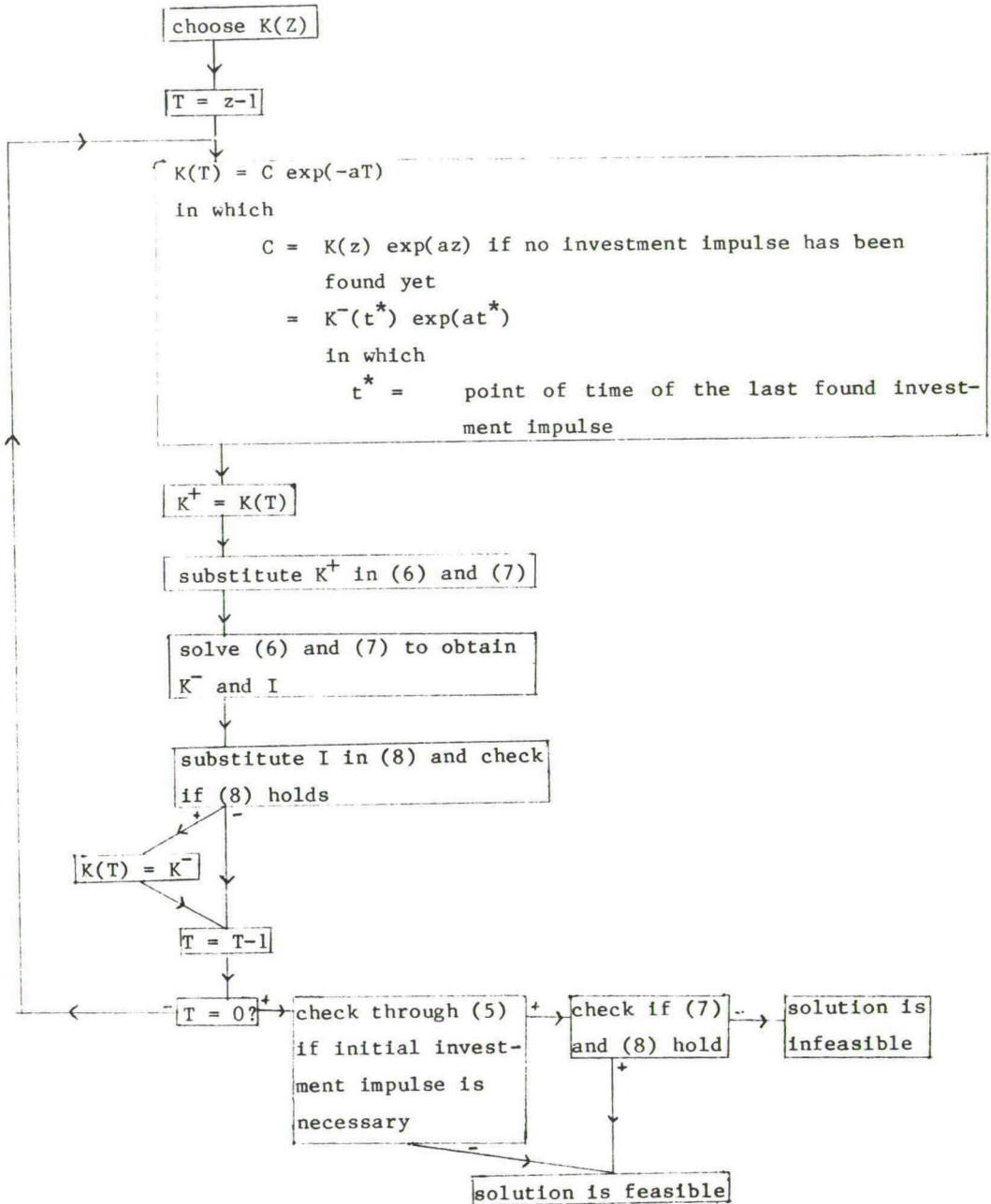
figure 4.1 the search procedure which enables us to develop the optimal investment pattern.
