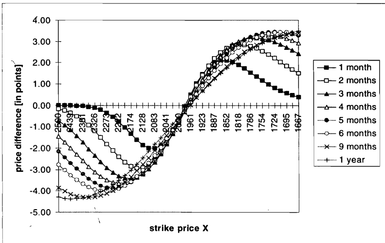
Figure 10: Deviation of EGARCH option prices [in points]
