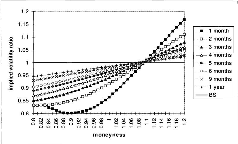
Figure 7: low initial volatility
