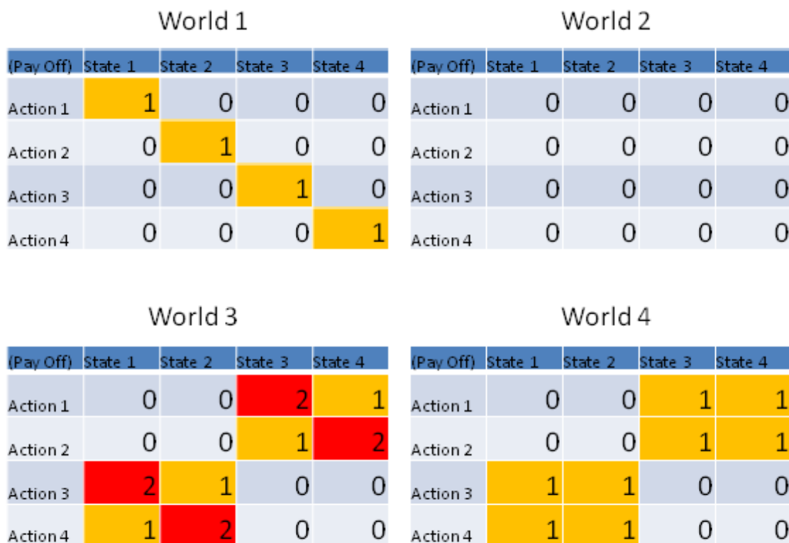
Figure 2. This figure depicts the relation between action and utility, given a certain world state. In world 1 the relevant information can be computed as two bits. The optimal strategy chooses a different action for every state of the world; therefore it has to obtain two bits of information to determine what state the world is in. World 2 is an example of a scenario
