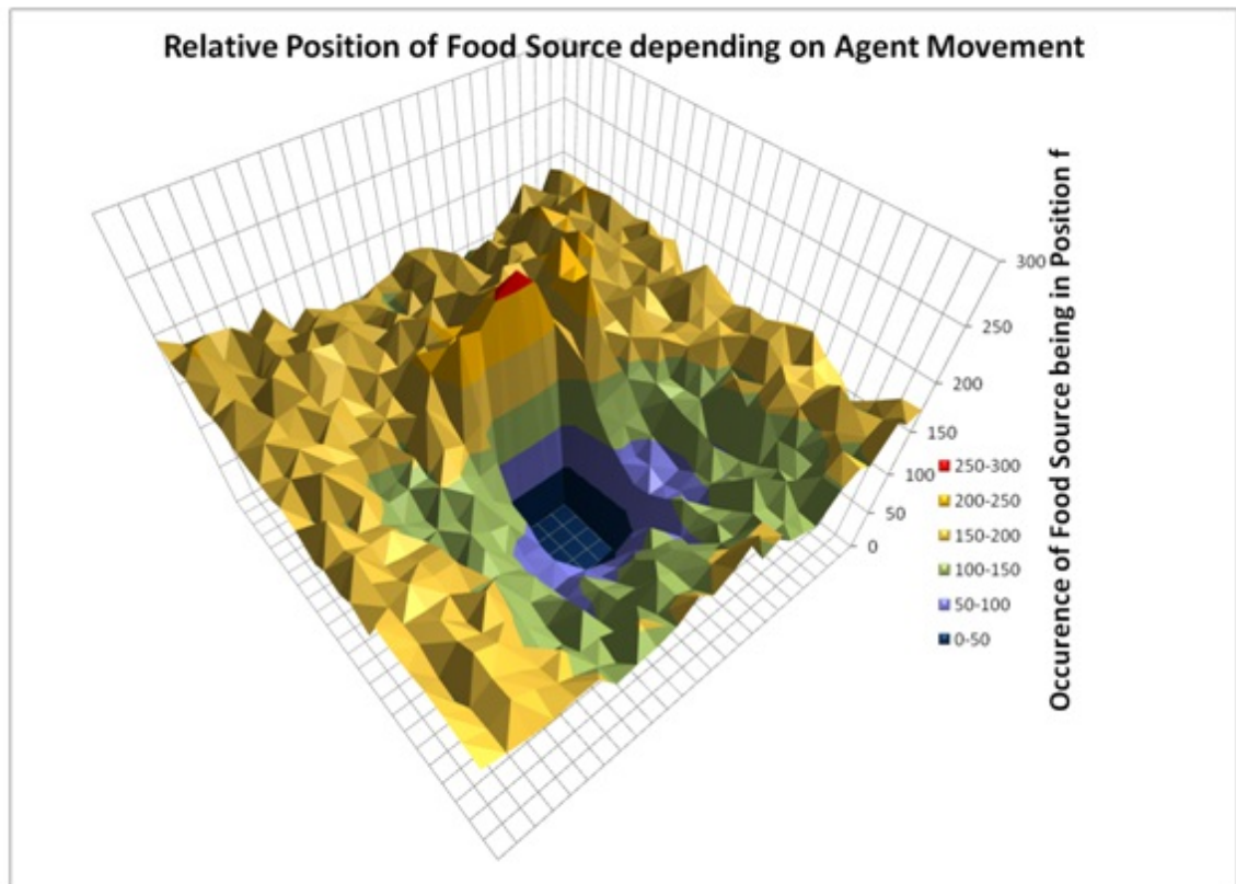
Figure 6. Graph showing P(FIA=\text{north}) , the distribution of F , the food source position, given a specific agent movement (in this case north). The data was obtained from 10000 single agent simulations. The position of the agent is in the center of the graph. Note that there is a peak north of the agent, meaning that it is more likely for the food source to be directly north of the agent when it moves north. Conversely, it is very unlikely for the food source to be in the southern sensor range while the agent moves north.
