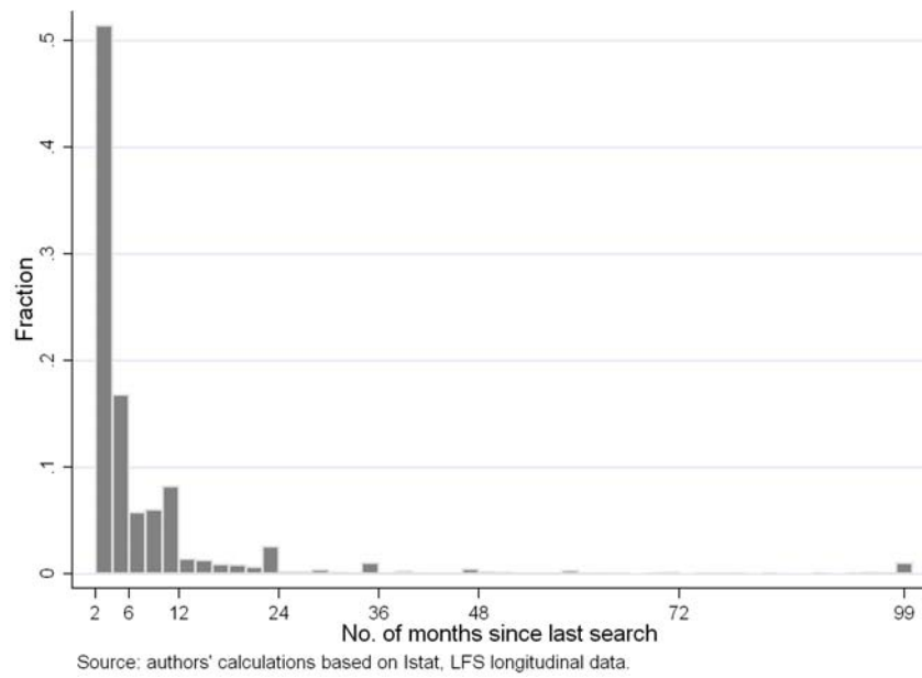
Figure 3: Distribution of the number of months since last search step in Italy
