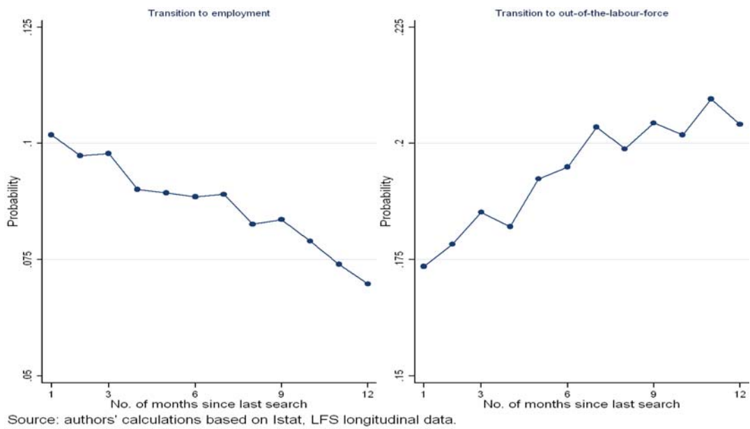
Figure 4: Quarterly transition probabilities by search intensity in Italy
