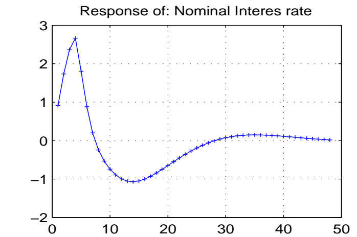
Figure 5: Impulse Responses to a Goods prices shock
