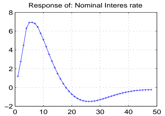
Figure 4: Impulse Responses to a Services prices shock
