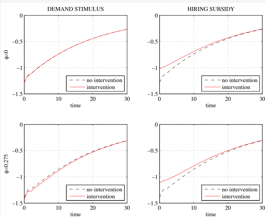
Figure 8 Response of GDP under a temporary increase in government spending (left column) and under a temporary subsidy to the cost of posting vacancies (right column) starting from a recession scenario for \phi = 0 (first row) and \phi = 0.275 (second row)
