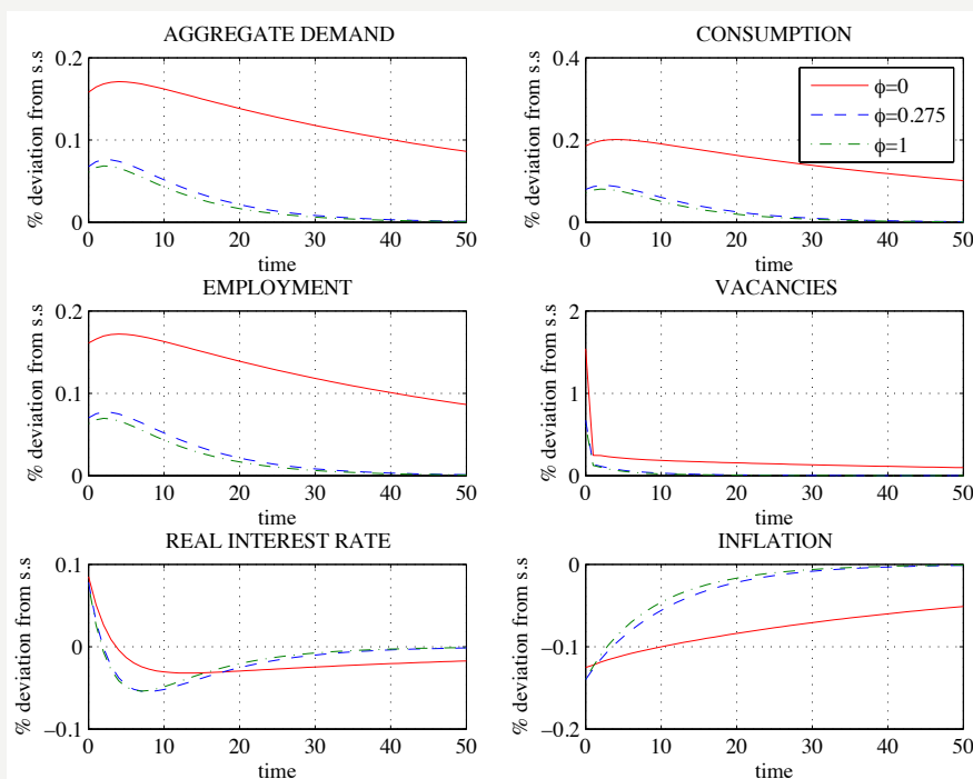
Figure 16 Impulse responses to a one percentage point temporary increase in the subsidy to the cost of posting vacancies using estimated parameters
