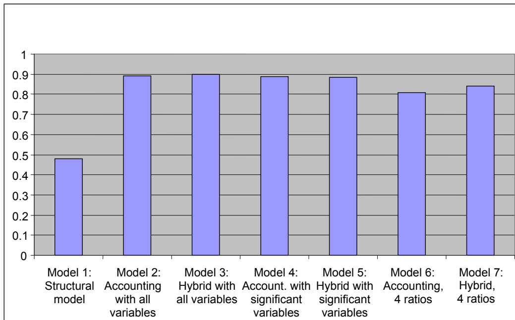
Figure 5: Accuracy ratio
