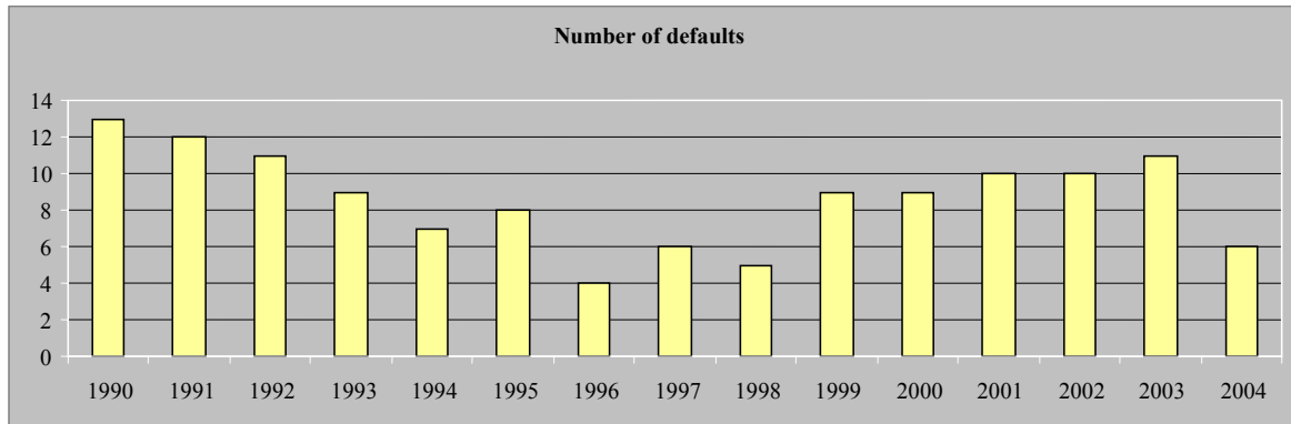
Figure 1: Distribution of defaults and reorganizations by year
