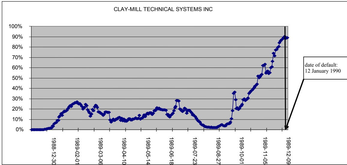
Figure 2: Daily default probabilities (1 year) of defaulting firms
