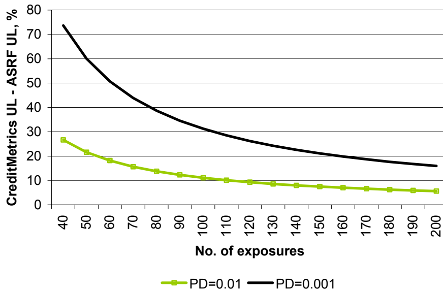
Figure 1: Convergence between CreditMetrics and ASRF
