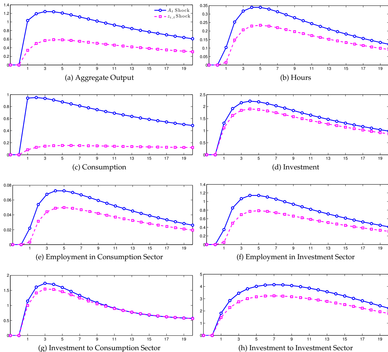
Figure 2: Responses to A_t and z_{i,t} Contemporaneous Shocks
