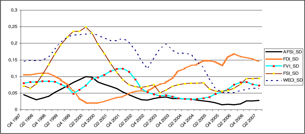
Figure 2: Standard deviation of FDI , FVI , FSI and WECI
