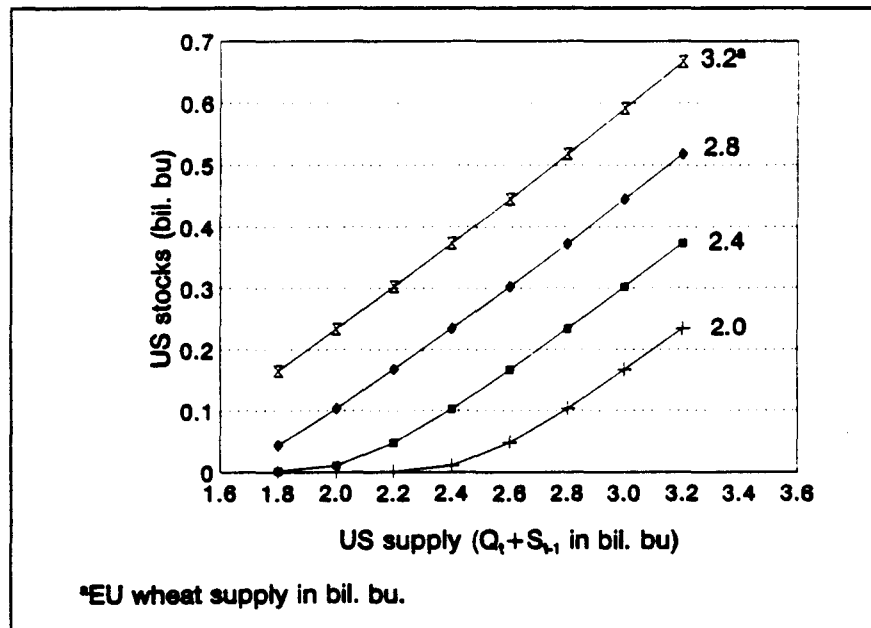
Figure 3. Equilibrium Storage Rules for US Wheat Under Alternative Supply Levels in the EU.
