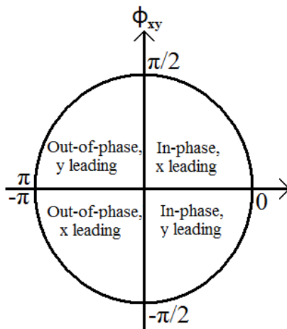
Figure 4: Phase-difference relations
